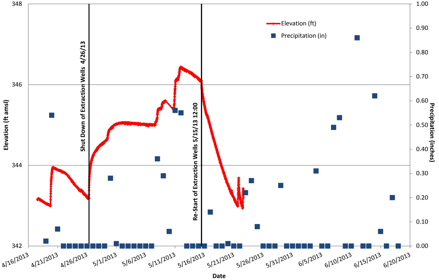
Figure 3.5-3 Building 2 Area MW-137A Vertical Extent Shutdown
